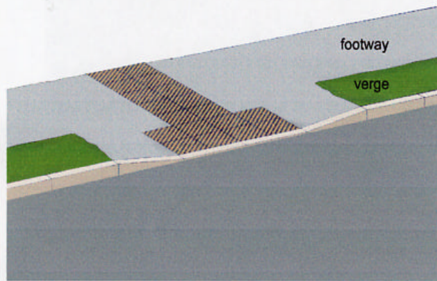
Tails to be provided where the crossing may be difficult to locate
