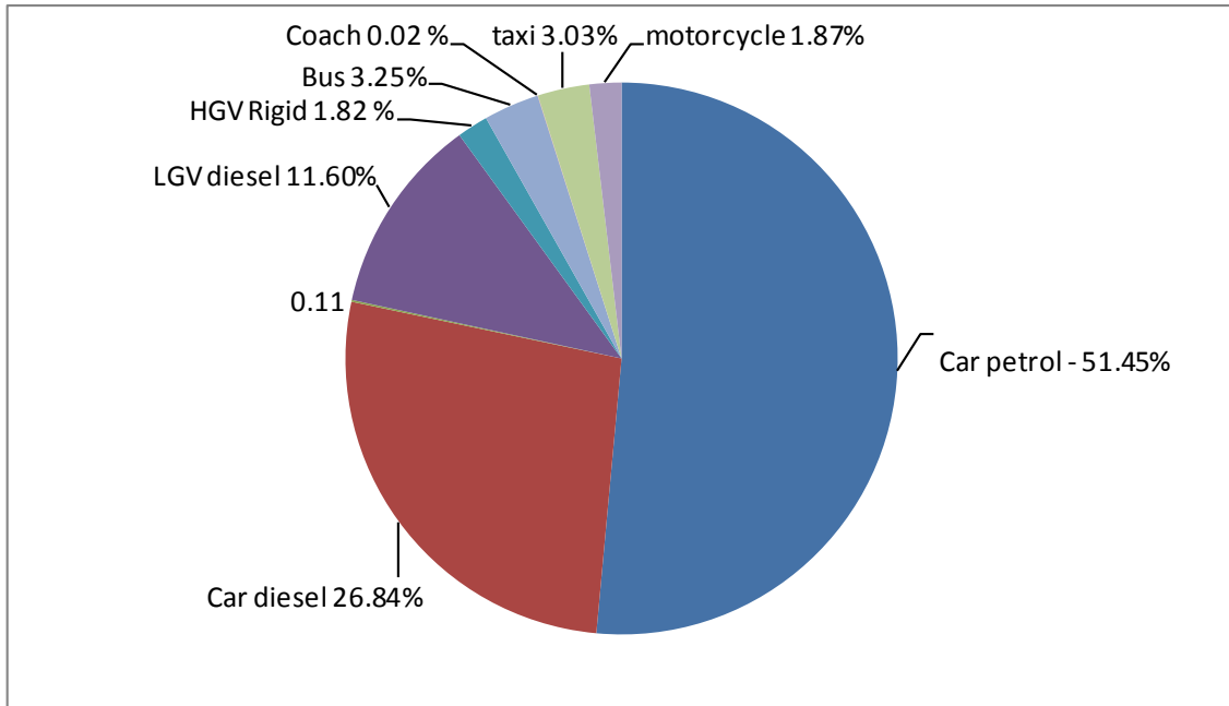
Figure 13: % contribution of individual vehicle types to total NO 2 from traffic in the Salisbury Terrace area
