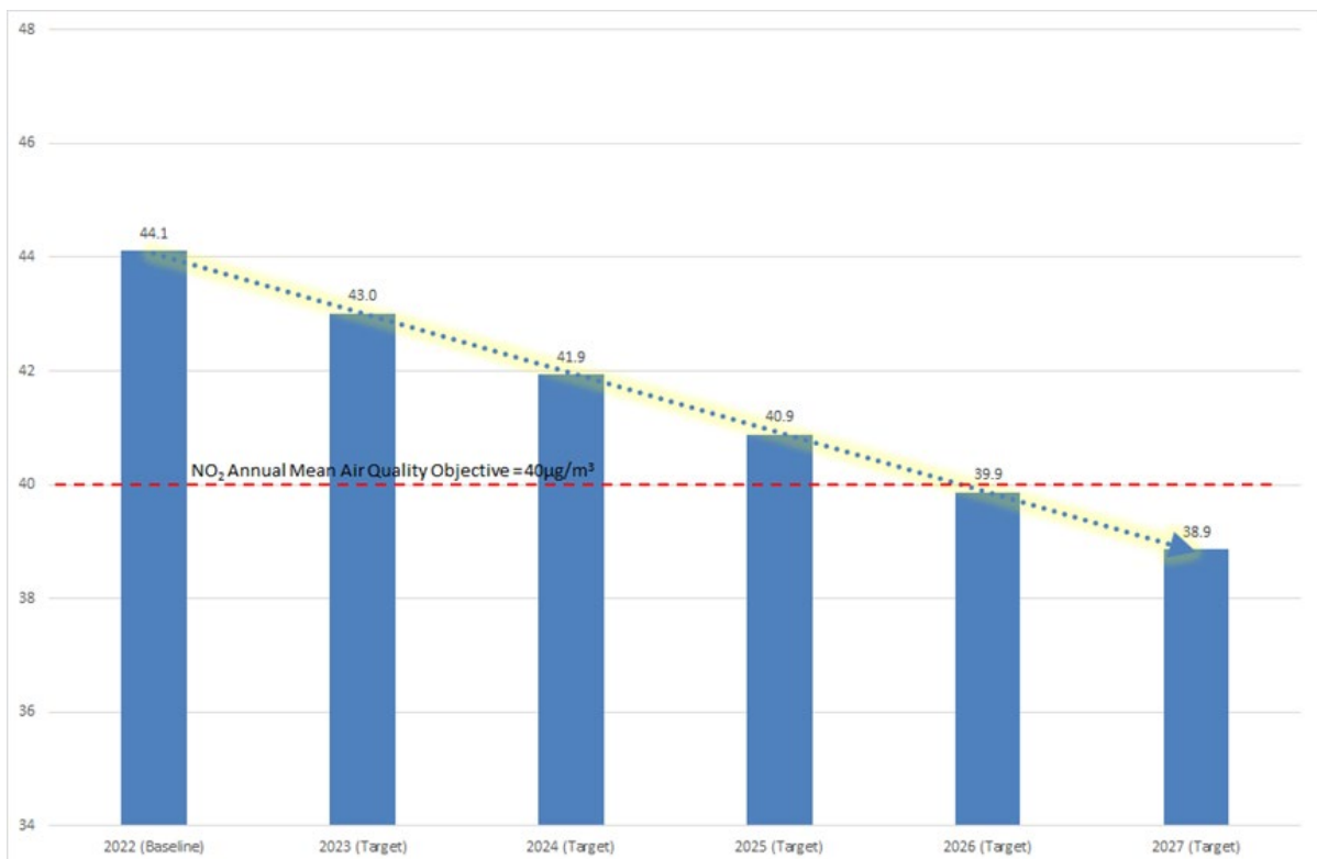
Figure 3-11 Air Quality 'Indicator 3' baseline (2022) and annual targets
