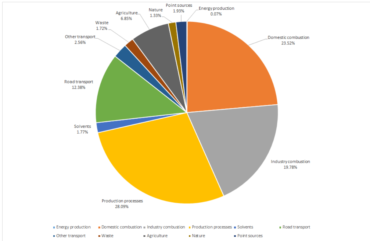
Figure 3-4 Source apportionment of NAEI sources of PM10 in CYC's Area
