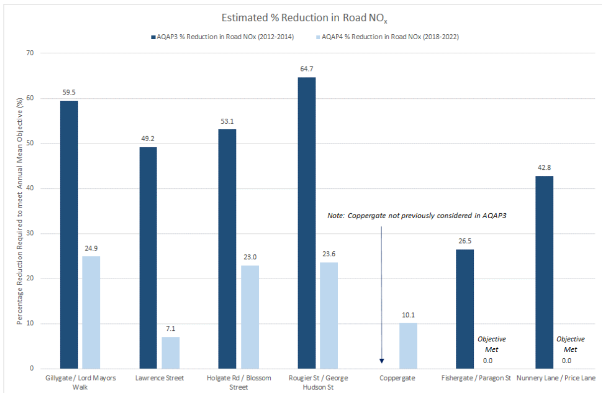
Figure 3-10 Percentage reduction in road NO x (AQAP3 vs AQAP4)
