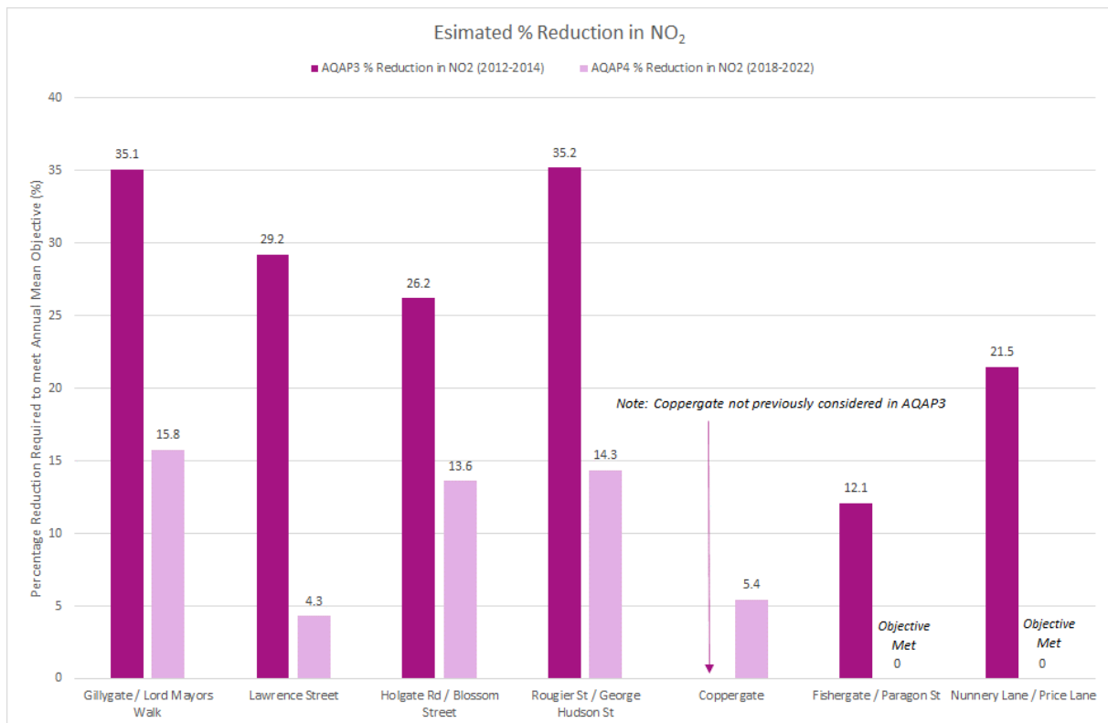
Figure 3-9 Percentage reductions in NO 2 (AQAP3 vs AQAP4)
