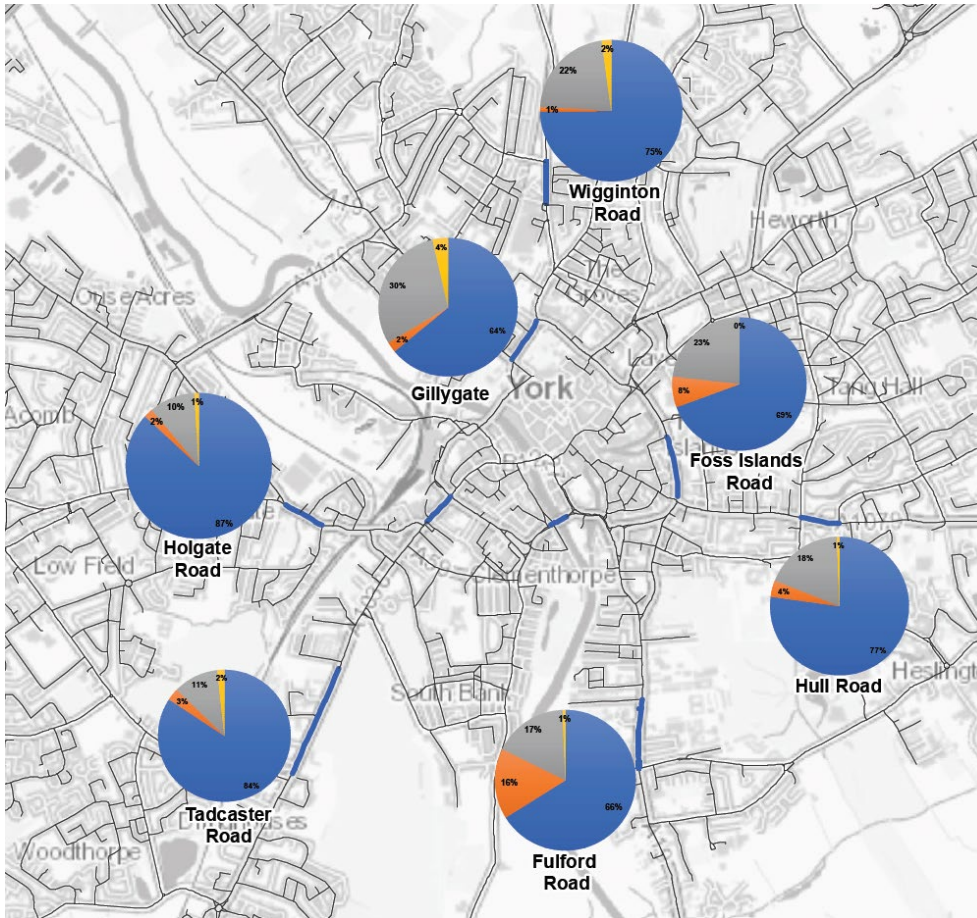
Figure 3-7 NOx emissions traffic source apportionment for selected roads
